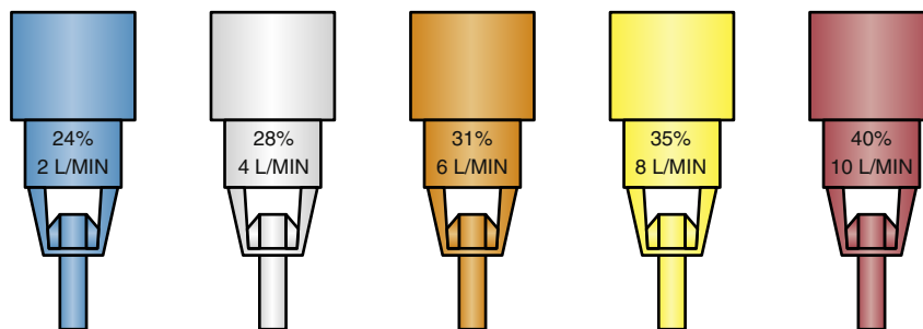
Interchangeable Venturi valves
